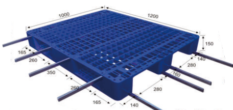
Model 型号: NA20# C-type Pallet (can place 8pcs steel pipe) Size 规格: 1200x1000x150mm
