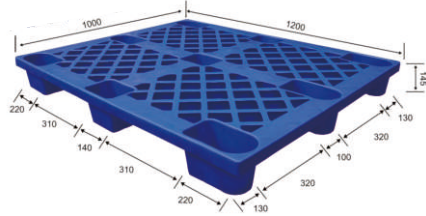
Model 型号: 1# 9 feel Pallet Size 规格: 1200x1000x145mm
